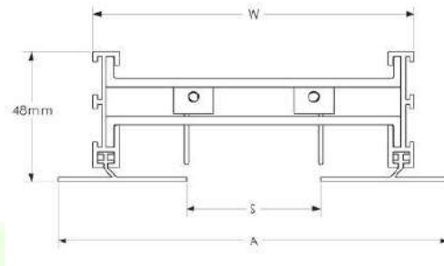
JET SLOT DIFFUSER- FLAT TYPE
