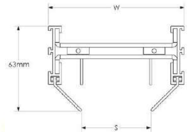
JET SLOT DIFFUSER- ANGULAR TYPE
